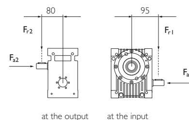
Bearing forces
