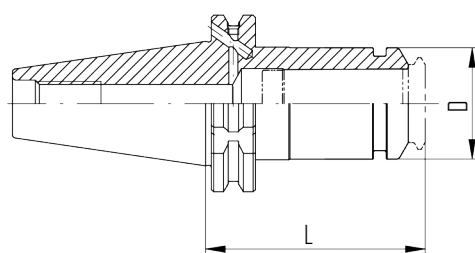
SK-B/PG (AD+B型)
